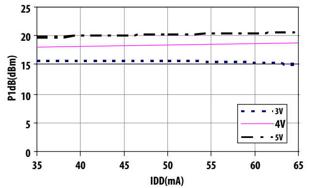
Figure 20. OP1dB vs IDD vs VDD
